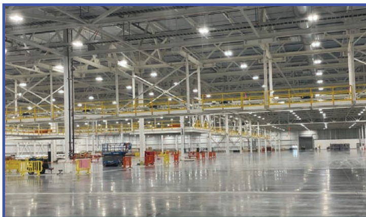
Ford's TEVC at BOC- Photo shows the body conveyors at the plant.
